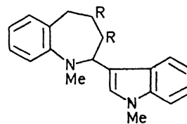
(8) R = \text{CO}_2\text{Me}
